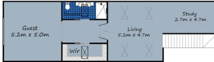
upper floor plan
